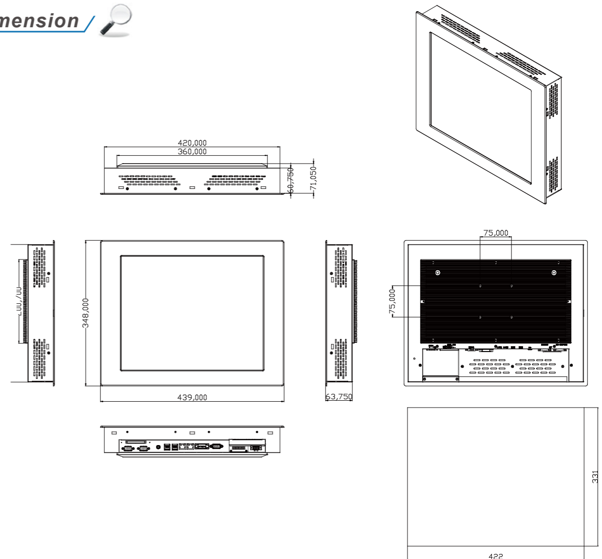
Mounting Hole
